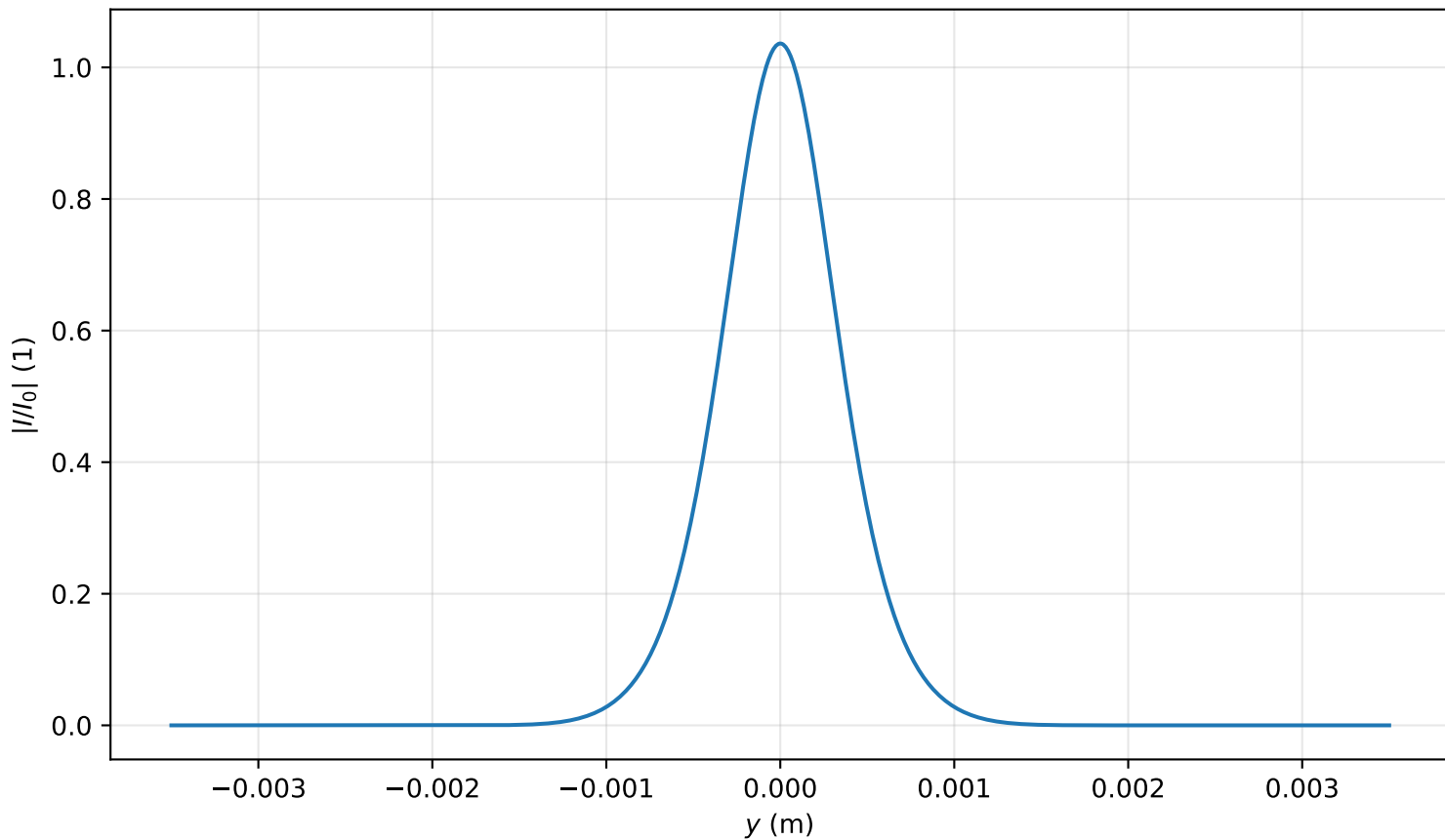
Intensity profile I(x=0, y, z=1.115)/I_0 , P_{in}=0.5P_{cr} , artificial time
